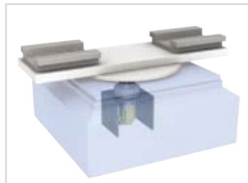
Pallet changer: rotary drive
