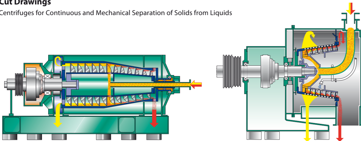
Decanter centrifuge with reducer type ZS
